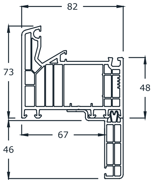
Art. 101.290.1 - telaio a ZETA 46
