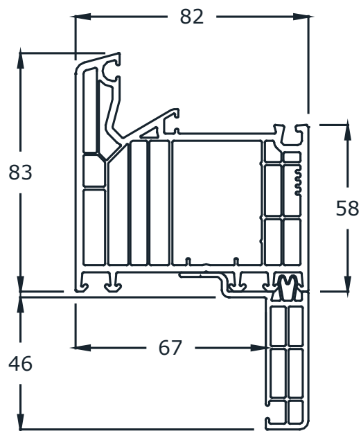
Art. 101.291.1 - telaio a ZETA 46
