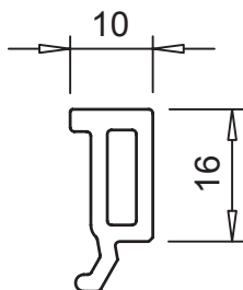
Art. 118.106 Fermapannello 10 mm
